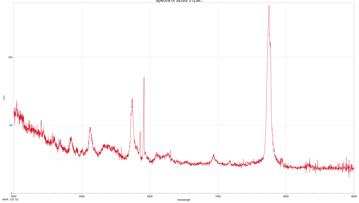
Spectra of SDSS J1236...
