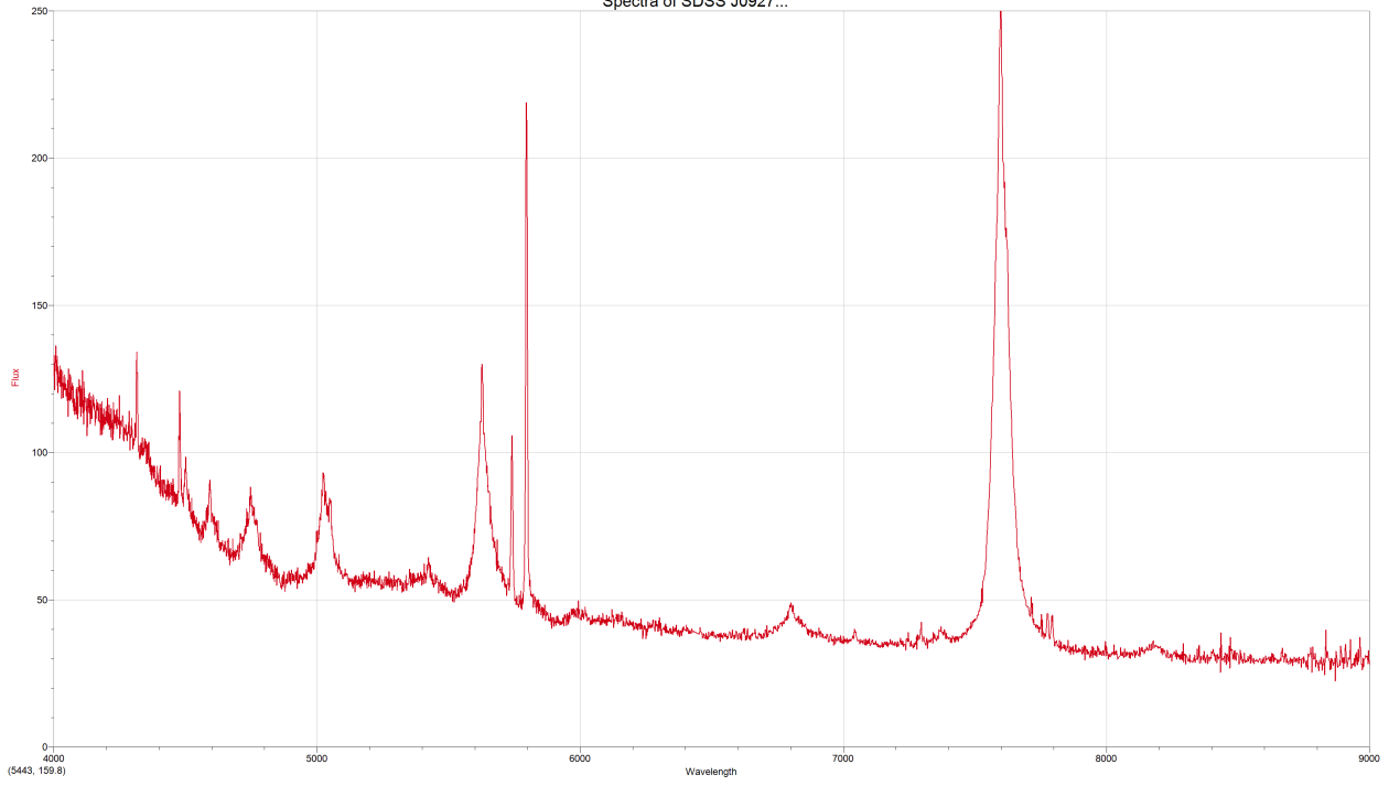
Spectra of SDSS J0927...
